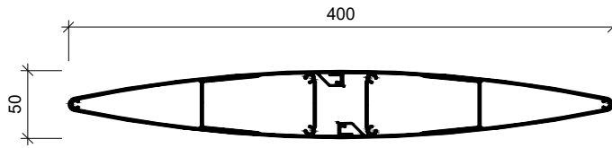
MF400 * EXTRUDED ALUMINIUM 2 PIECE BLADE
