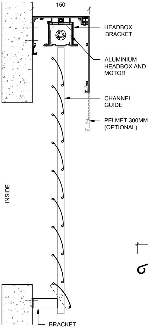
MV80CC BLADE
