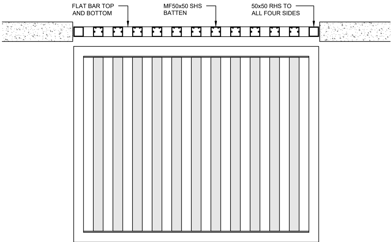
MF50x50 SHS BATTEN - REVEAL FIXED
