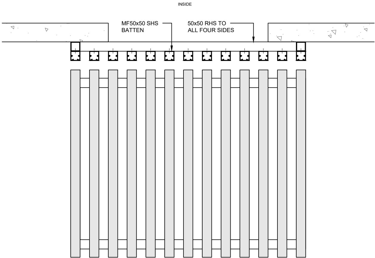
MF50x50 SHS BATTEN - FACE FIXED
