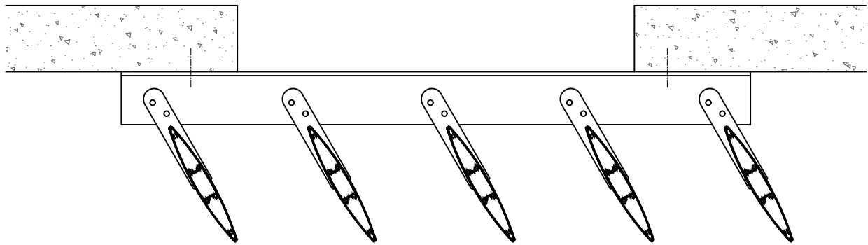
PLAN VIEW (MF200 WITH FORK BRACKET * ) (FINS CAN BE IN OPPOSITE DIRECTION AS SHOWN)
