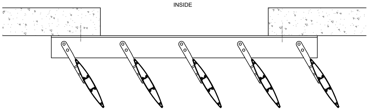
INSIDE PLAN VIEW (MF200 WITH TEARDROP BRACKET * ) (FINS CAN BE IN OPPOSITE DIRECTION AS SHOWN)
