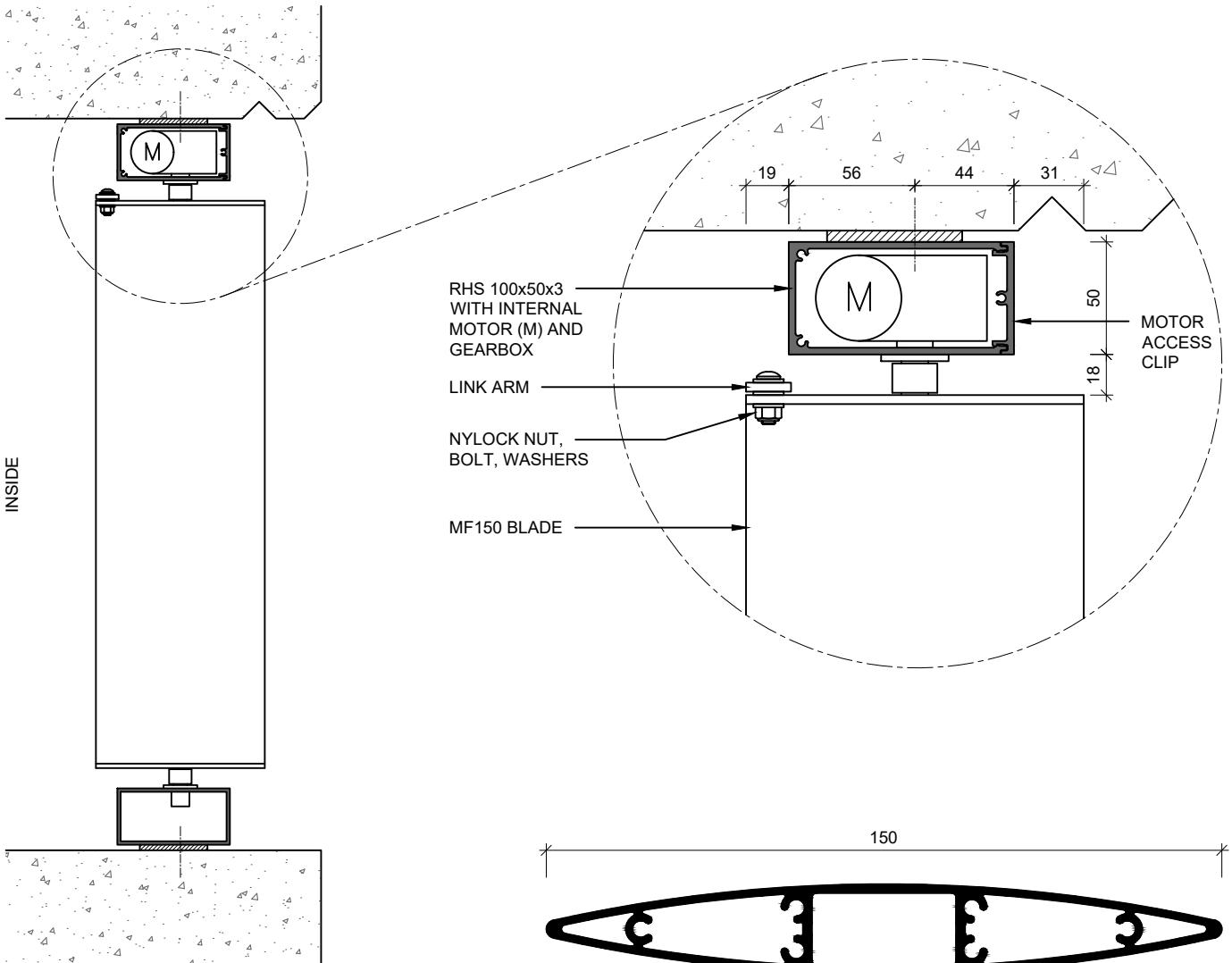
PLAN VIEW (BLADES MOUNTED VERTICALLY) (FINS CAN BE IN OPPOSITE DIRECTION AS SHOWN)
