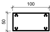
MF100x50 - RHS EXTRUDED ALUMINIUM
