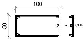
MF100x50 - RHS EXTRUDED ALUMINIUM 2 PIECE
