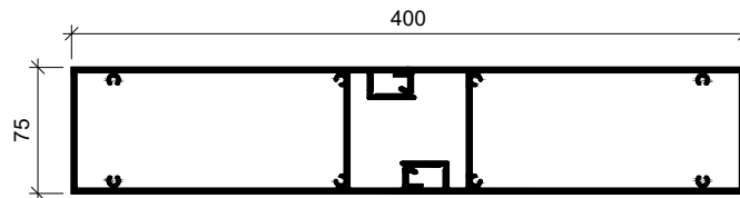
MF400x75 - RHS * EXTRUDED ALUMINIUM 2 PIECE
