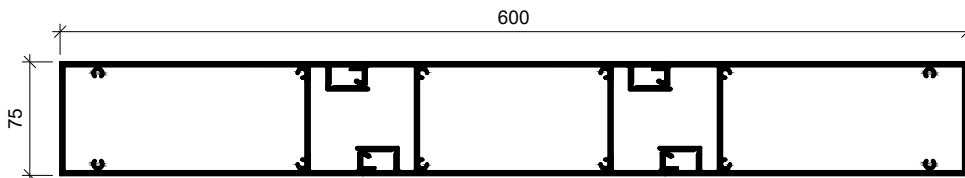
MF600x75 - RHS * EXTRUDED ALUMINIUM 3 PIECE
