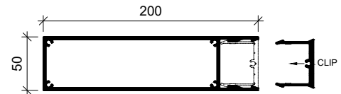
MF200x50 - RHS * EXTRUDED ALUMINIUM
