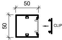
MF50x50 - SHS BATTEN EXTRUDED ALUMINIUM 2 PIECE
