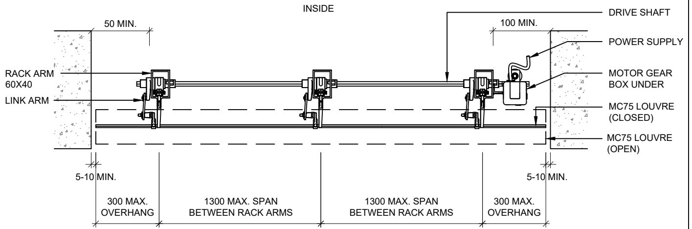
PLAN VIEW (LOUVRES INSIDE REVEAL)
