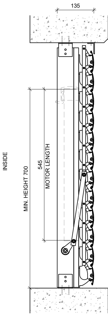
SECTION (LOUVRES CLOSED)
