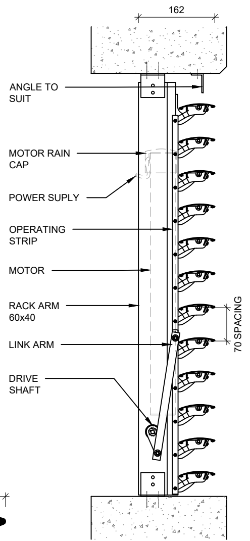
SECTION (LOUVRES OPENED)
