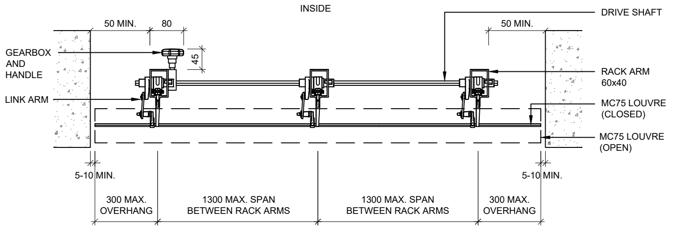
PLAN VIEW (LOUVRES INSIDE REVEAL)
