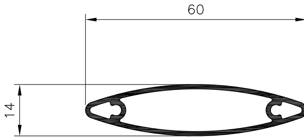
MS60 SHUTTER BLADE EXTRUDED ALUMINIUM
