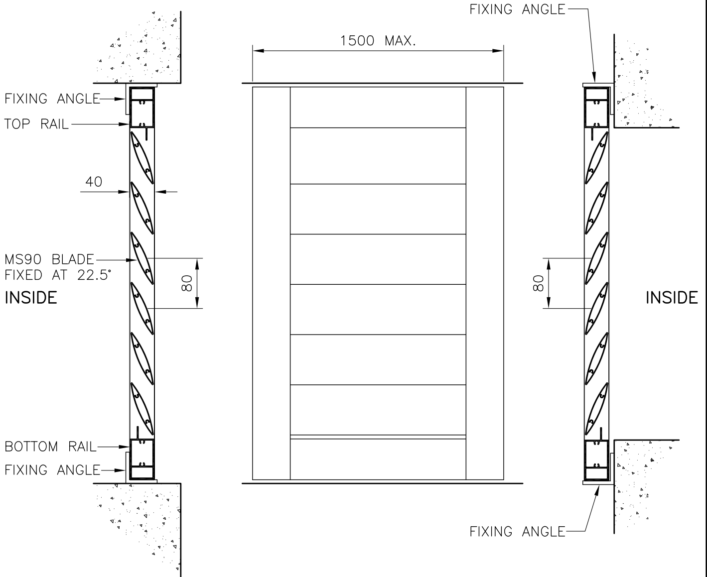
SECTION REVEAL FIXING
