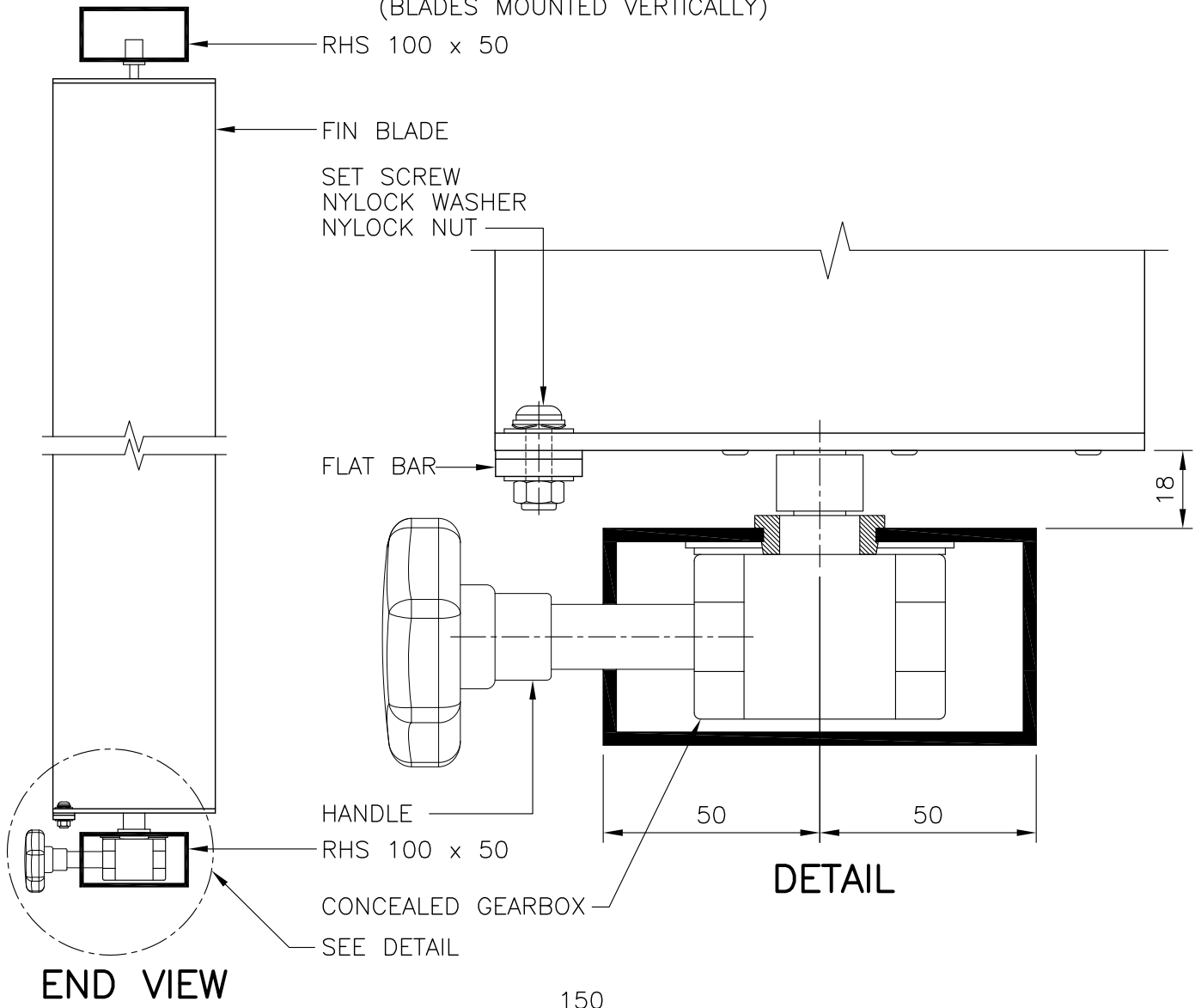
PLAN SECTION (BLADES MOUNTED VERTICALLY)
