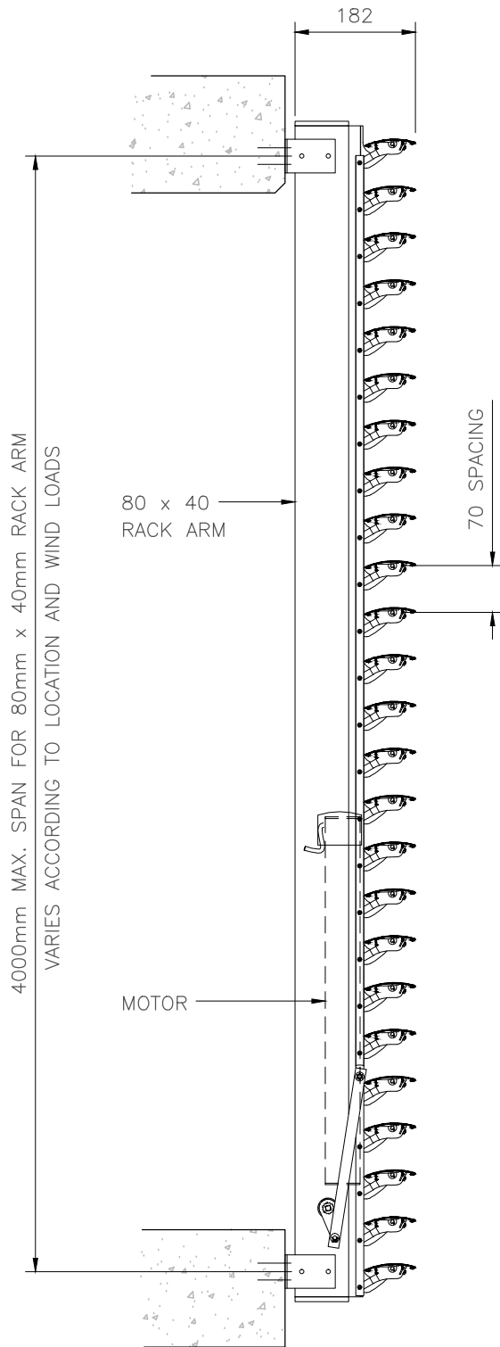
80mm x 40mm RACK ARMS
