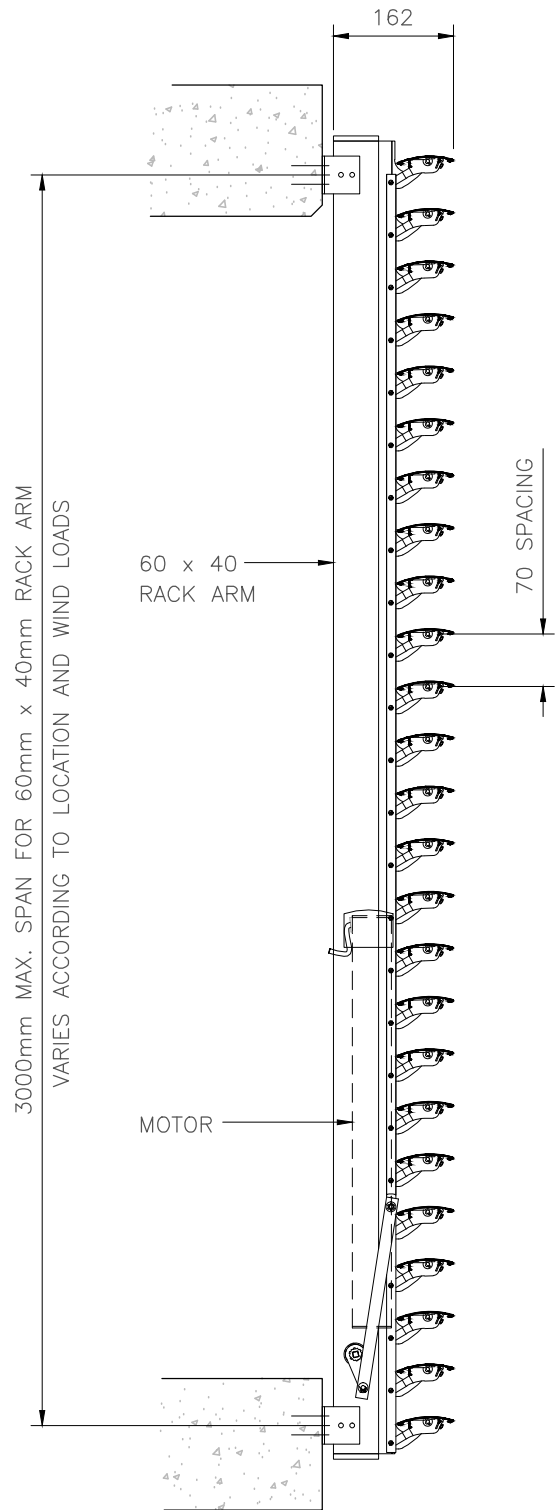
60mm x 40mm RACK ARMS
