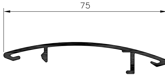
MC75 CONTINUOUS LOUVRE EXTRUDED ALUMINIUM
