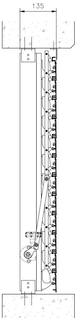
SIDE VIEW (LOUVRES CLOSED)
