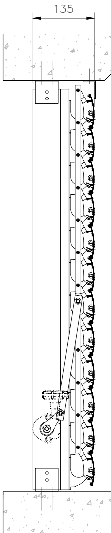
SIDE VIEW (LOUVRES CLOSED)
