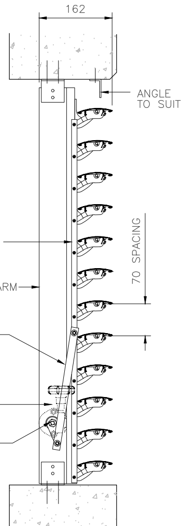
SIDE VIEW (LOUVRES OPEN)
