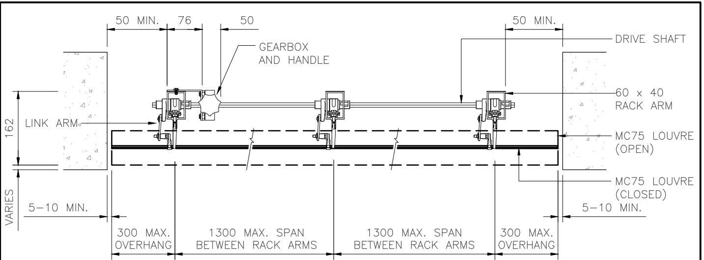
PLAN VIEW LOUVRES INSIDE REVEAL
