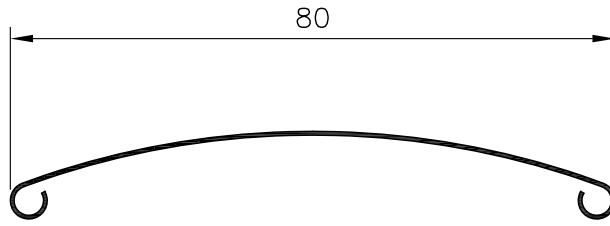
MV80C EXTERNAL VENETIAN ALUMINIUM
