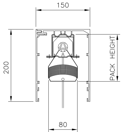
RETRACTED BLIND
