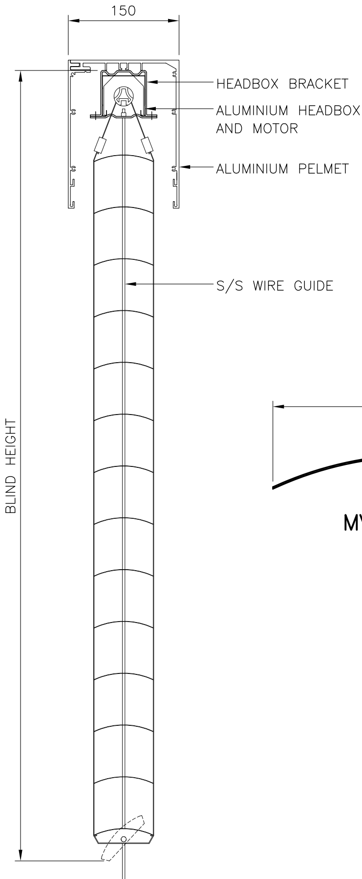
EXTENDED BLIND
