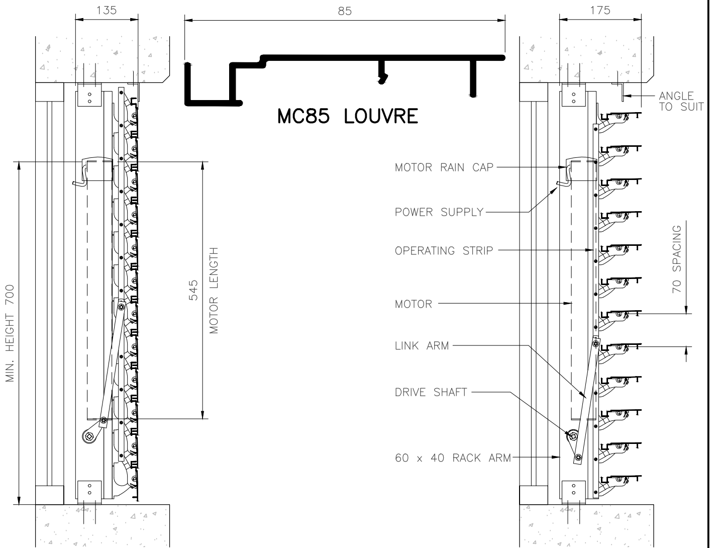
SIDE VIEW (LOUVRES CLOSED)
