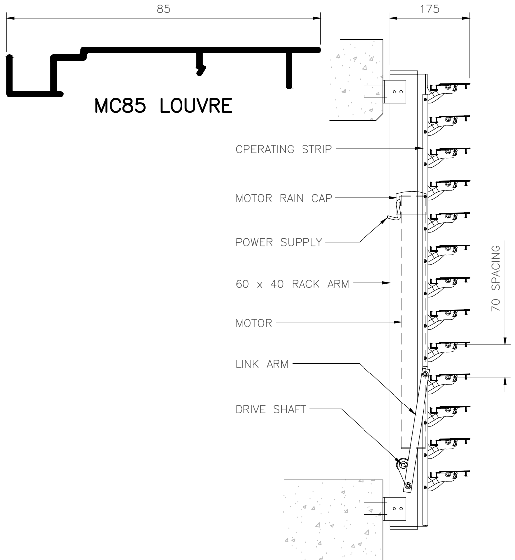
SIDE VIEW (LOUVRES OPEN)
