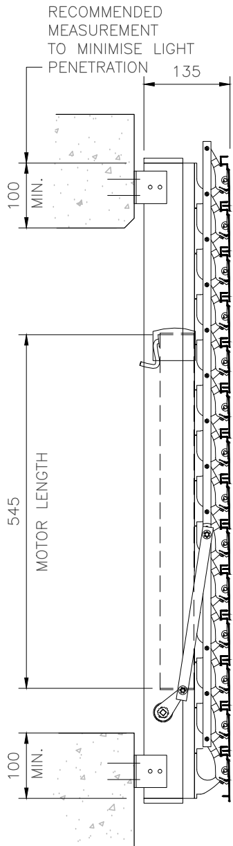
SIDE VIEW (LOUVRES CLOSED)
