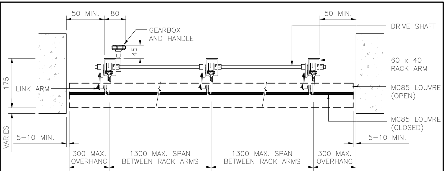
PLAN VIEW LOUVRES INSIDE REVEAL
