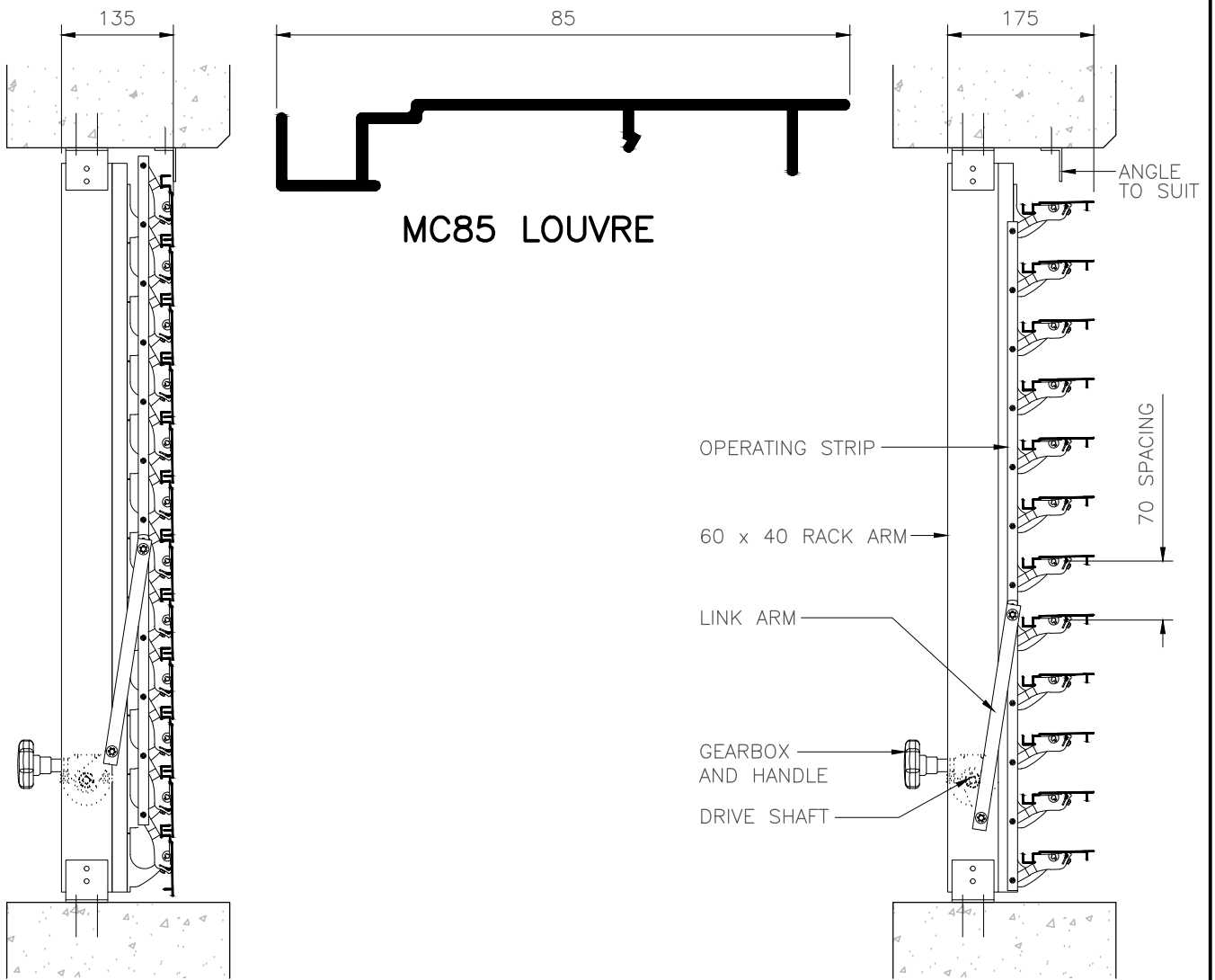
SIDE VIEW (LOUVRES CLOSED)
