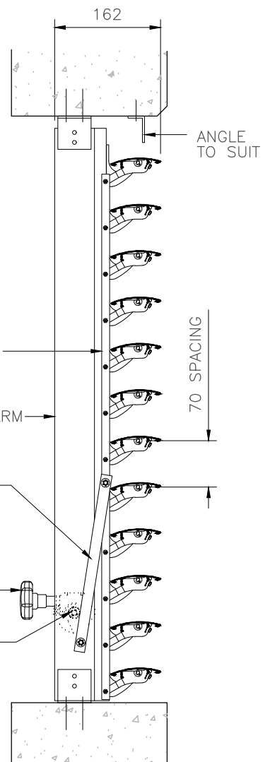
SIDE VIEW (LOUVRES OPEN)
